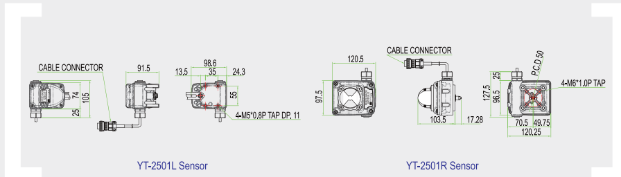
YT-2501 Body
