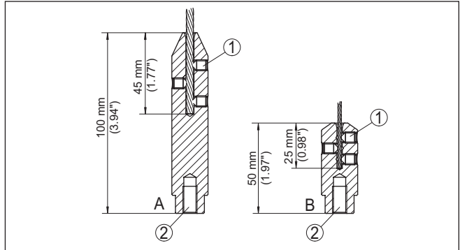
插图. 24: 截短缆式电极
